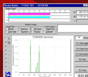
Frequency Spectrums
