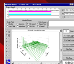
Waterfall Plots
