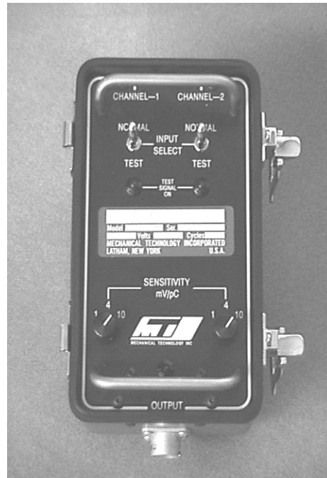
Model 8000-4225 Charge Amplifier
