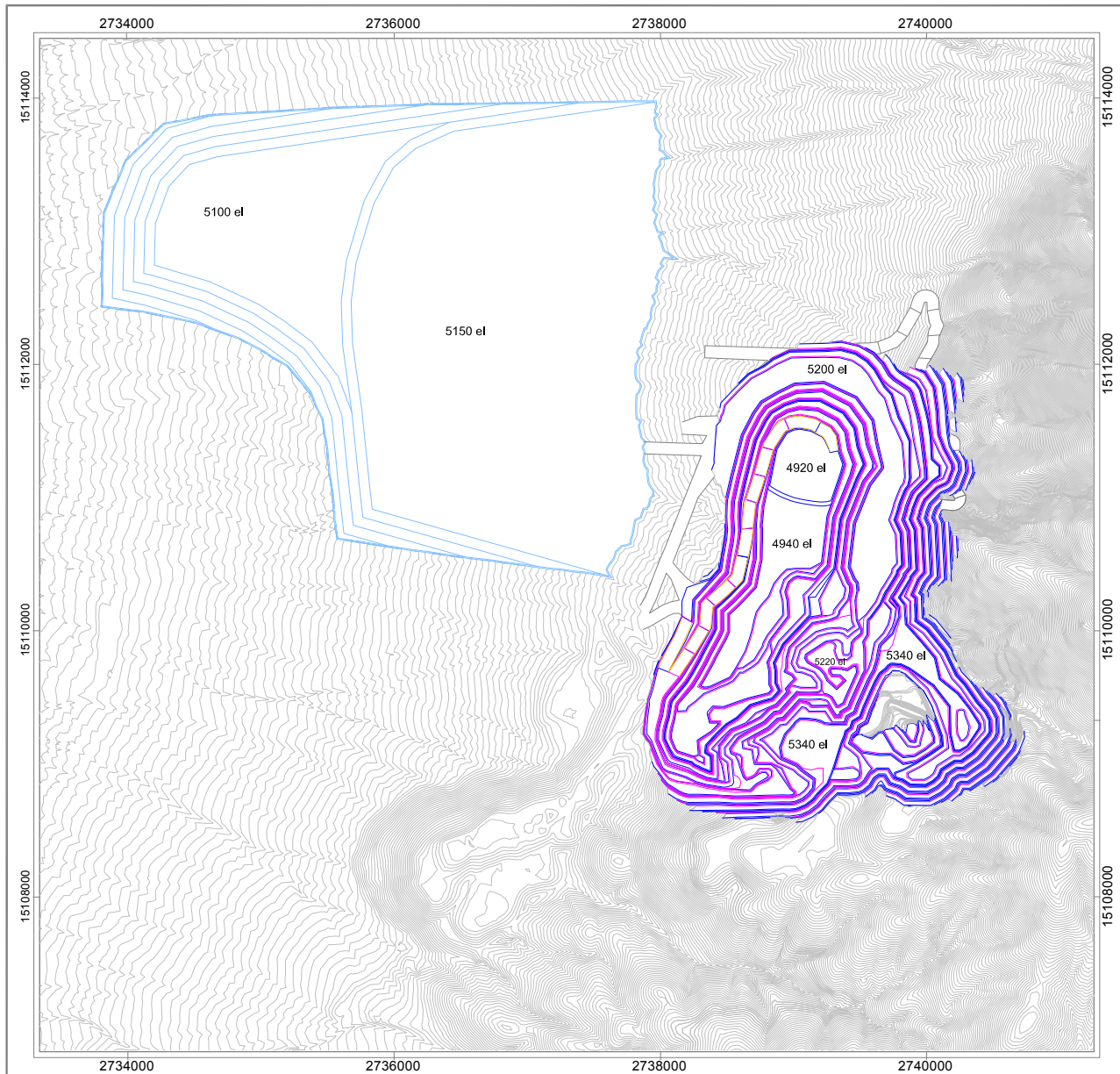
Figure 16.9 Year 3 Pit and Waste Dump Design
