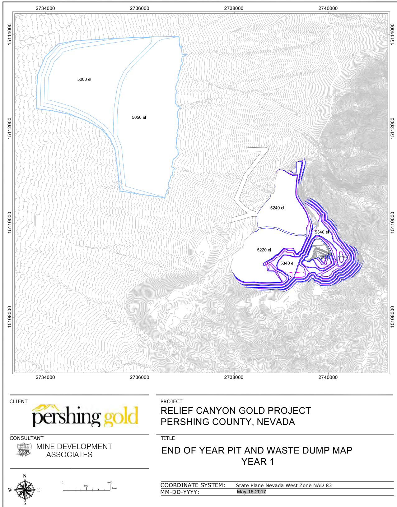
Figure 16.7 Year 1 Pit and Waste Dump Design
