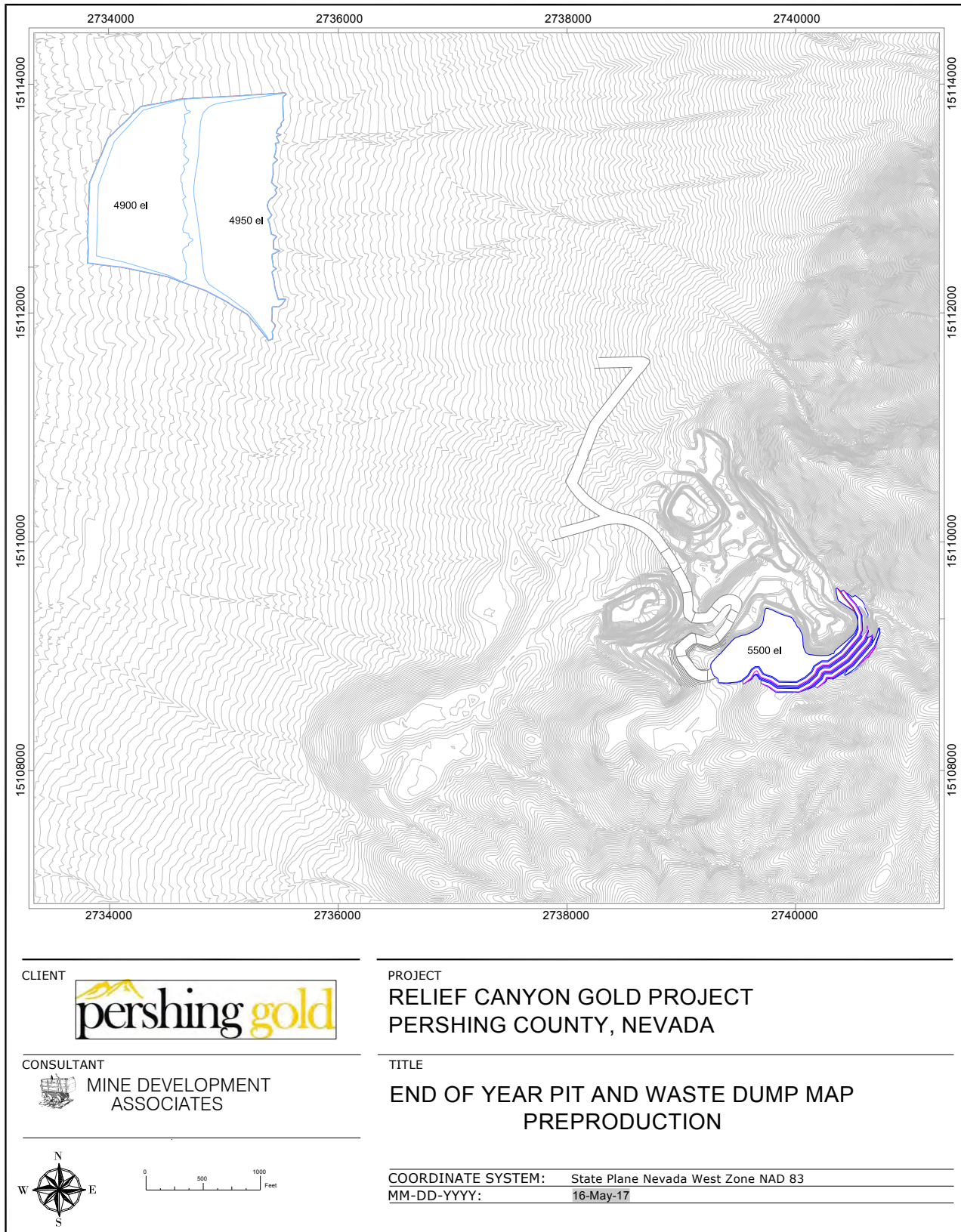
Figure 16.6 Pre-production Pit and Waste Dump Design
