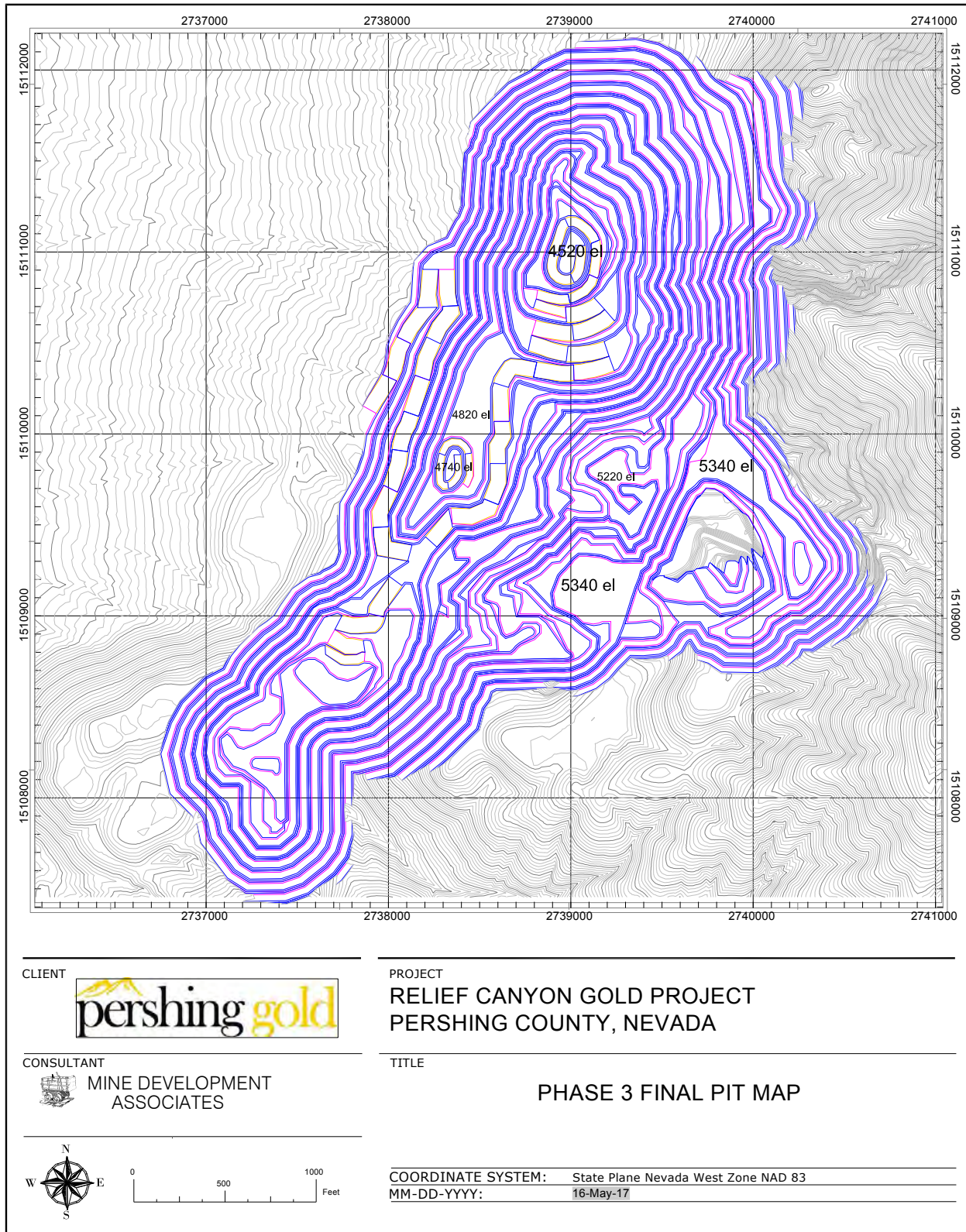
Figure 16.5 Final Pit Design
