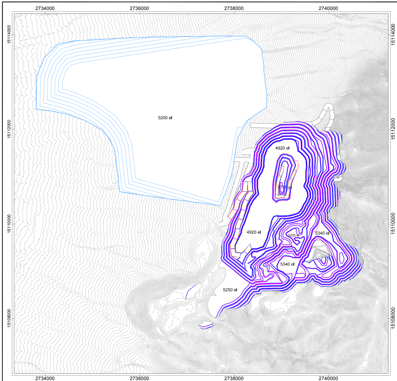
Figure 16.10 Year 4 Pit and Waste Dump Design
