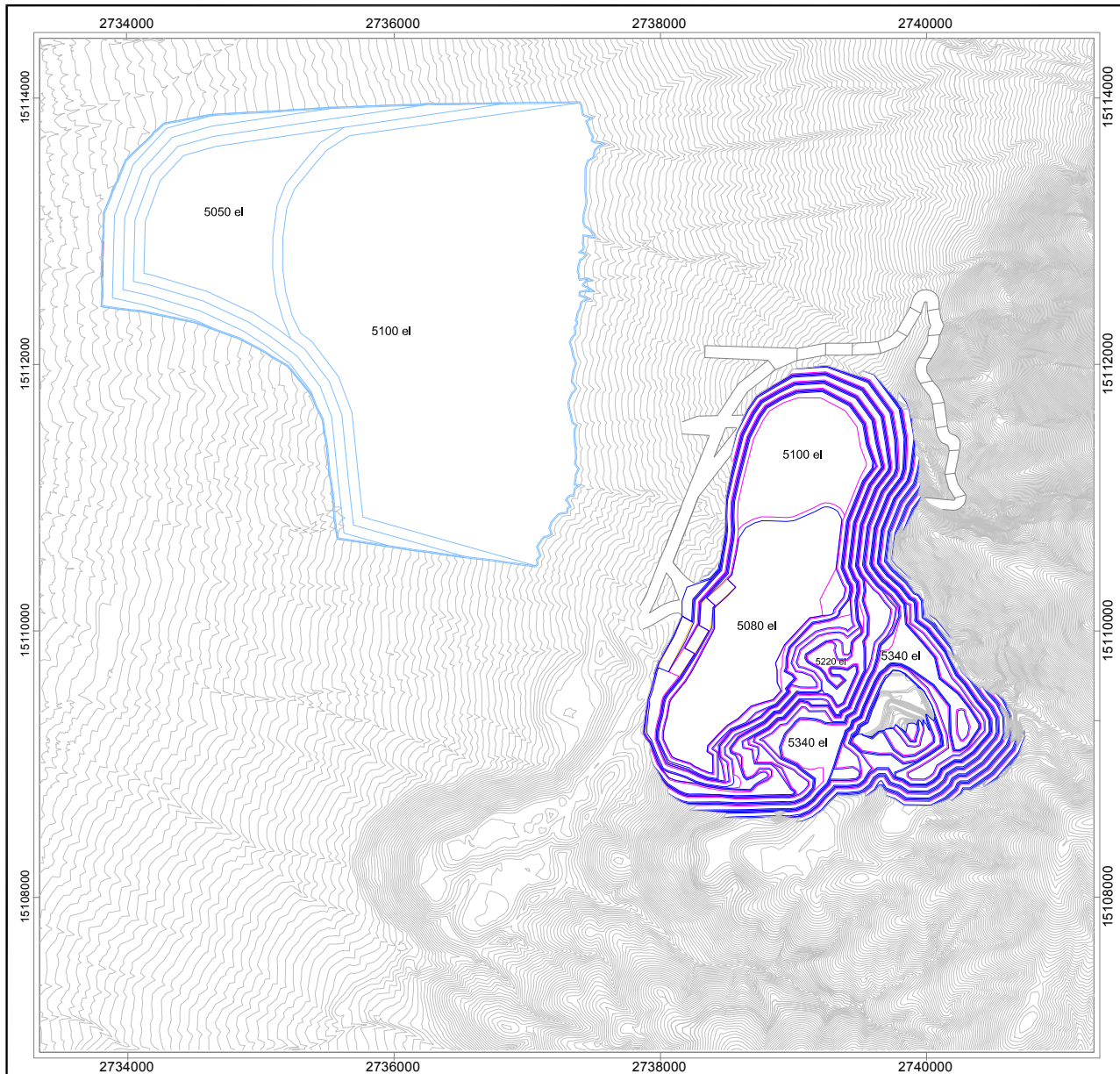
Figure 16.8 Year 2 Pit and Waste Dump Design
