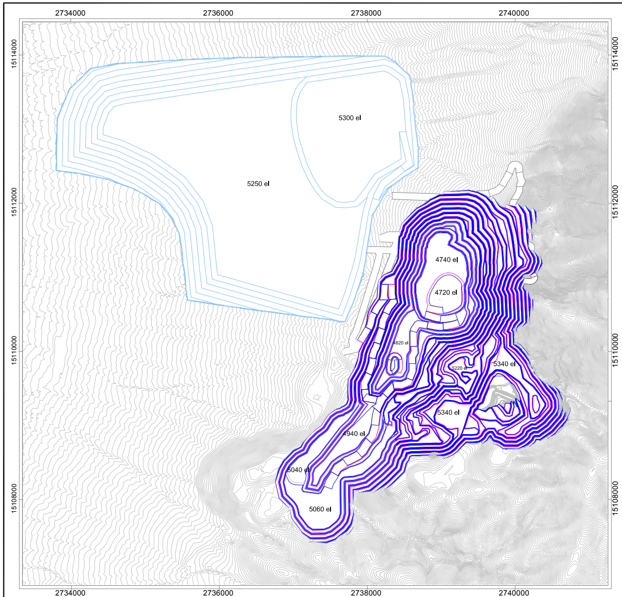
Figure 16.11 Year 5 Pit and Waste Dump Design
