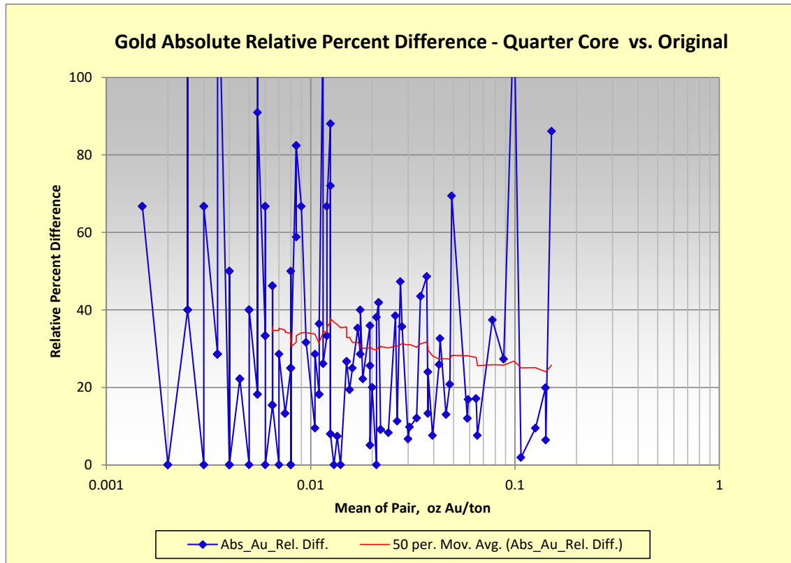
Figure 11.6 Quarter-Core Duplicate Analyses– Absolute Relative Difference
