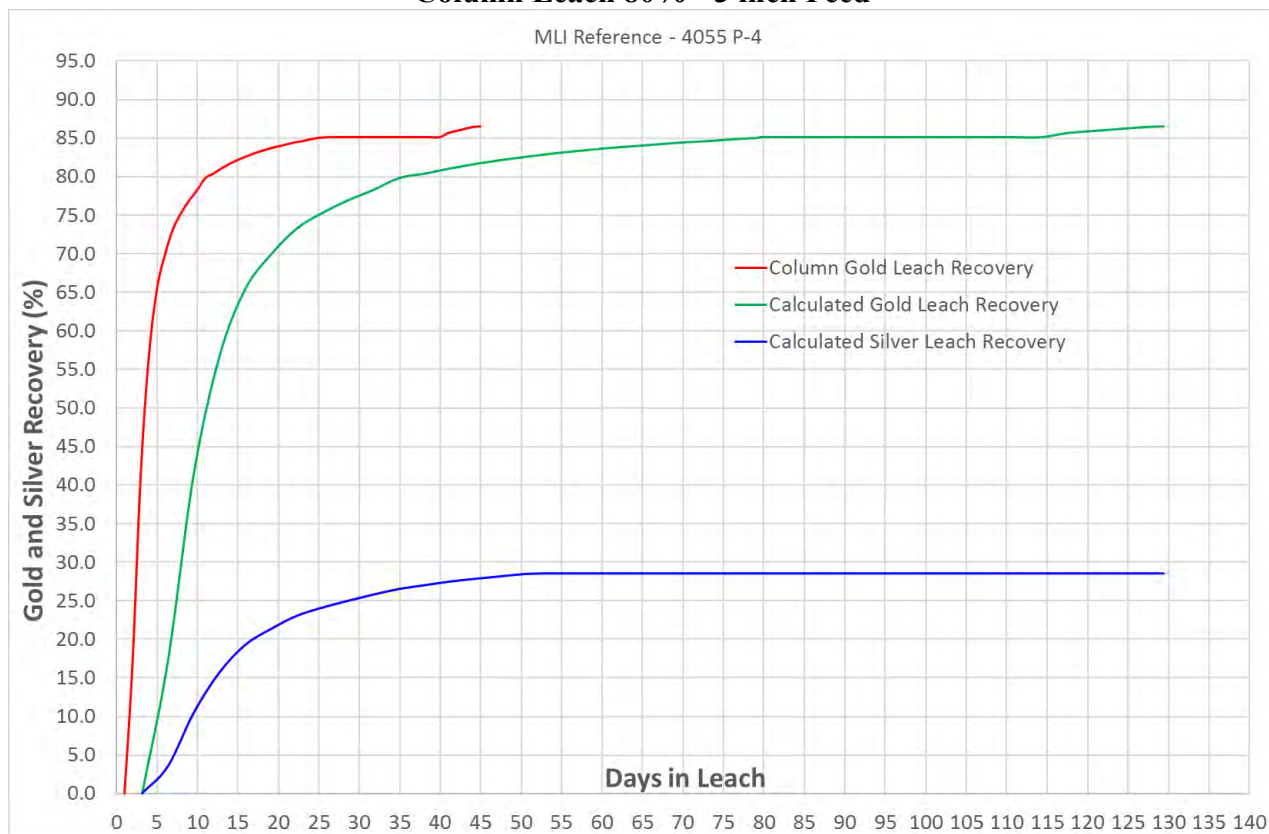
Figure 13.9 Leach Rate Profiles, Bulk Sample BS-2-NC 70/30 Low Fines High Fines Mix Column Leach 80% - 3 inch Feed
