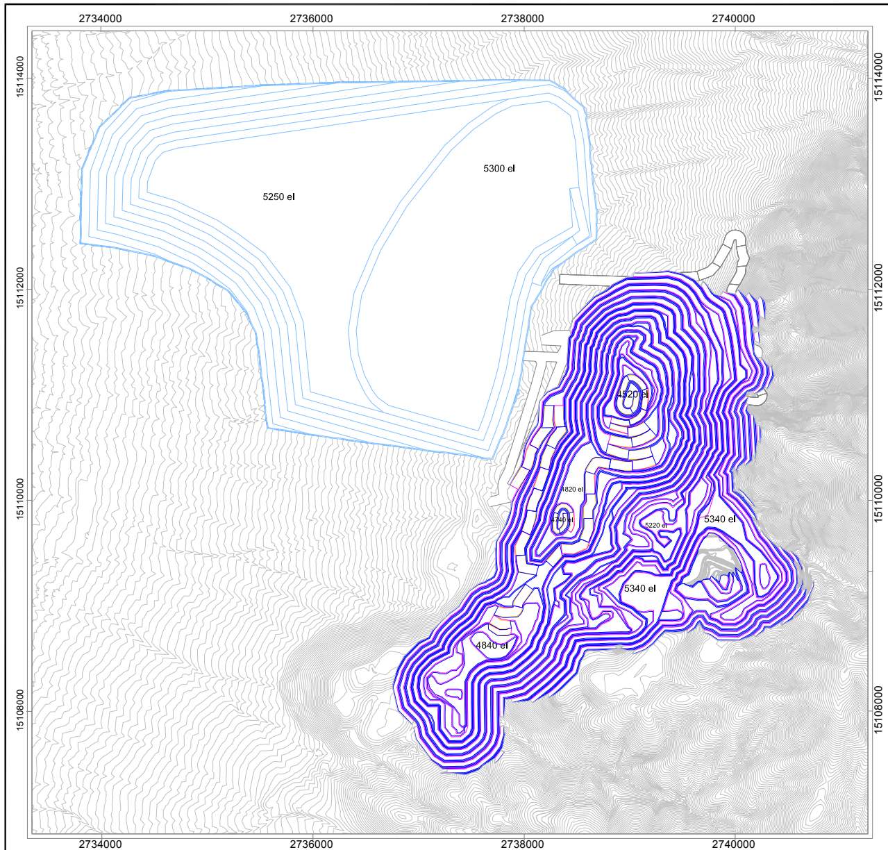
Figure 16.12 Year 6 Final Pit and Waste Dump Design
